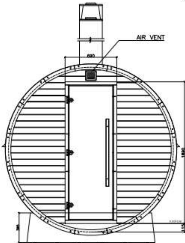
FRONT ELEVATION 1/10 SCALE
