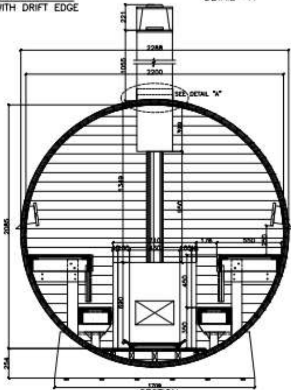
SECTION 1/10 SCALE
